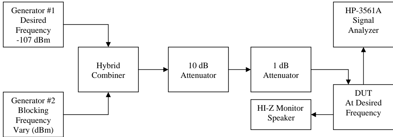
Fig. 5-7 — Blocking Dynamic Range Test Hook-up
