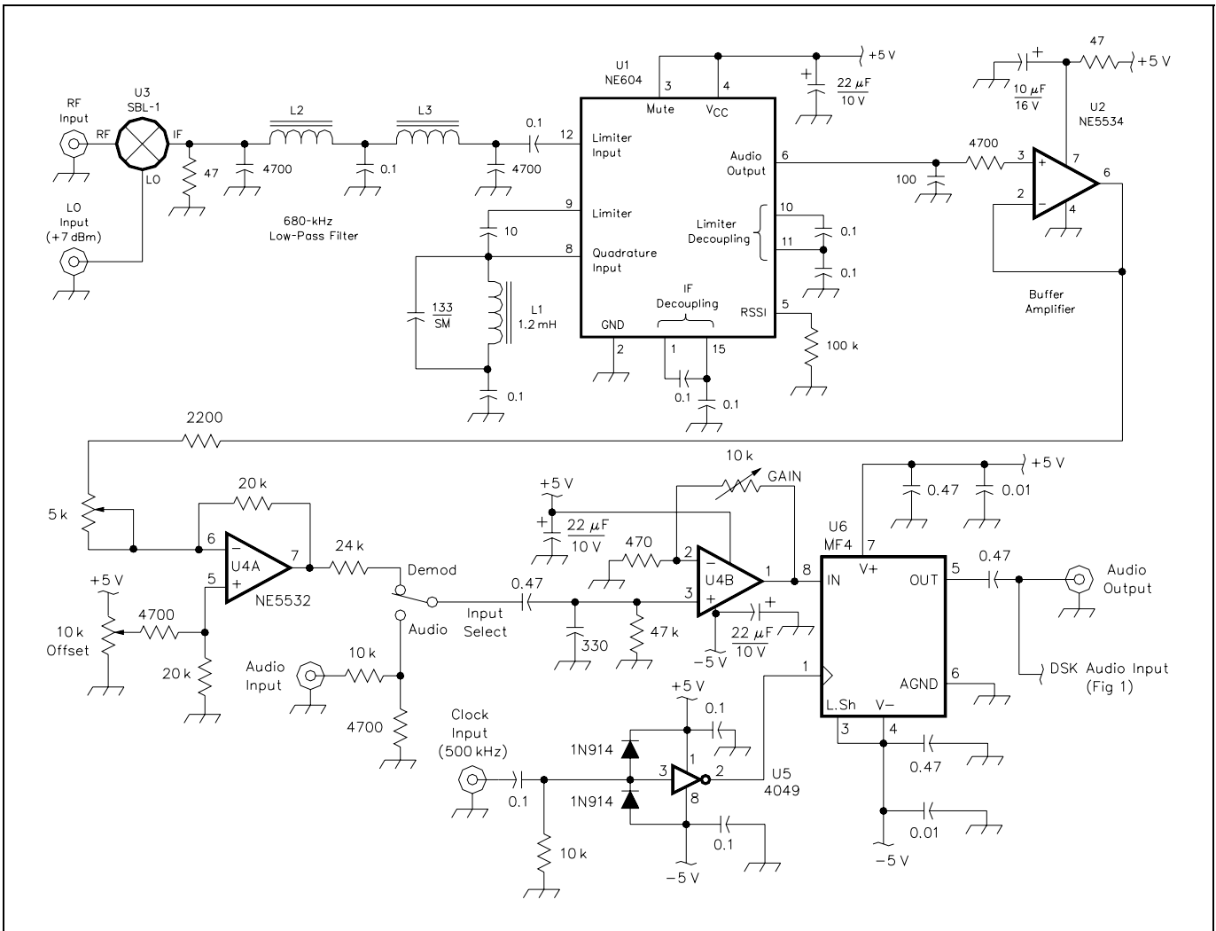
Fig 2 -- Schematic diagram of the BER test box circuit. L1 -- 1.2-mH Toko 10RB fixed inductor. (Digi-Key part TK4401-ND.) L2, L3 -- 41 turns #28 enam wire on a T-50-1 toroid core.
