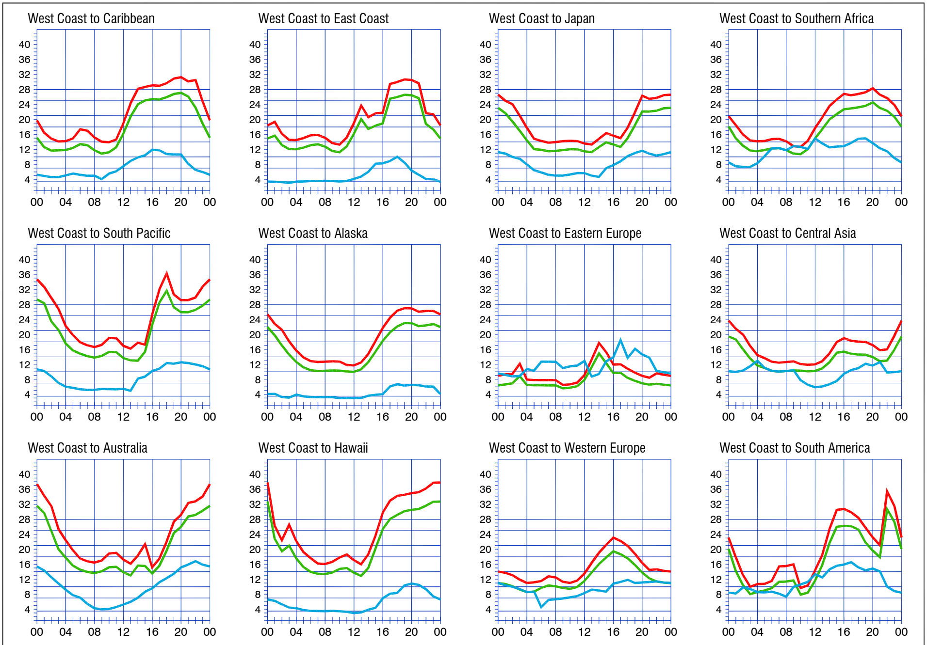
When are the bands open? These charts, generated using CAPman, show probabilities for average HF propagation in the month of October for the paths indicated. The horizontal axes show Coordinated Universal Time (UTC), and the vertical axes frequency in MHz. On 10% of the days of this period, the highest frequencies propagated will be at least as high as the upper red curves (HPF, highest possible frequency) and on 50% of the days they will be at least as high as the green curves (MUF, classical maximum usable frequency). The blue curves show the lowest usable frequency (LUF) for a 1500-W CW transmitter. For SSB or a lower transmitter power, the LUF will be somewhat higher than the blue curves indicate. See Oct 1994 QST , pp 27-30, and Feb 1995 QST , pp 34-36, for more details. The predictions assume an observed 2800-MHz solar flux value of 79. This is a Very Low level of solar activity. See the detailed propagation tables on The ARRL Antenna Book CD-ROM .
