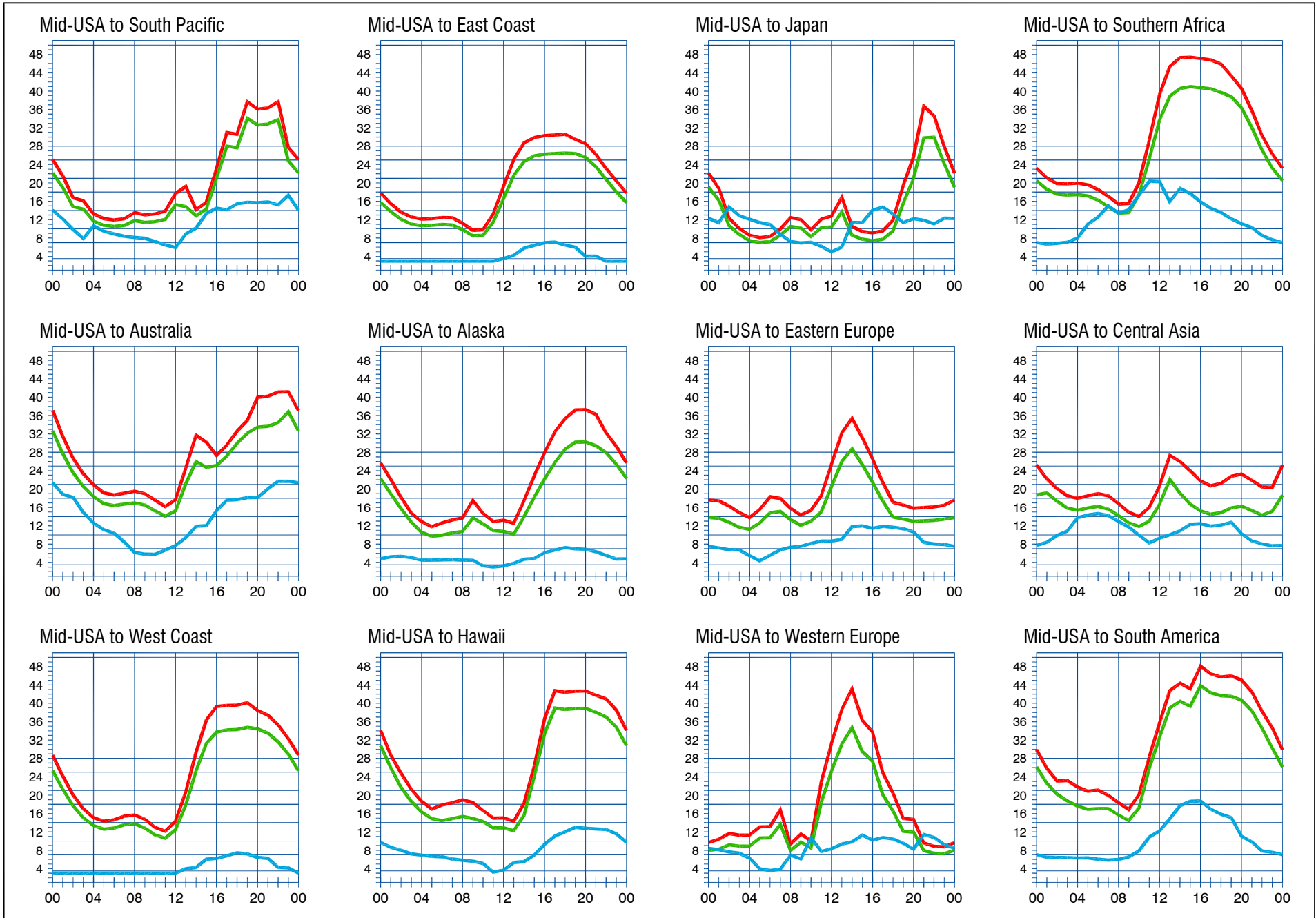
When are the bands open? These charts, generated using CAPman, show probabilities for average propagation in the Month of November. On 10% of the days of this period, the highest frequencies propagated will be at least as high as the upper red curves (HPF, highest possible frequency) and on 50% of the days they will be at least as high as the green curves (MUF, classical maximum usable frequency). The blue curves show the lowest usable frequency (LUF) for a 1500-W CW transmitter. For SSB or a lower power transmitter, the LUF will be somewhat higher than the blue curves indicate. The horizontal axes show Coordinated Universal Time (UTC) and the vertical axes frequency in MHz. These predictions assume an observed 2800-MHz solar flux value of 146.
