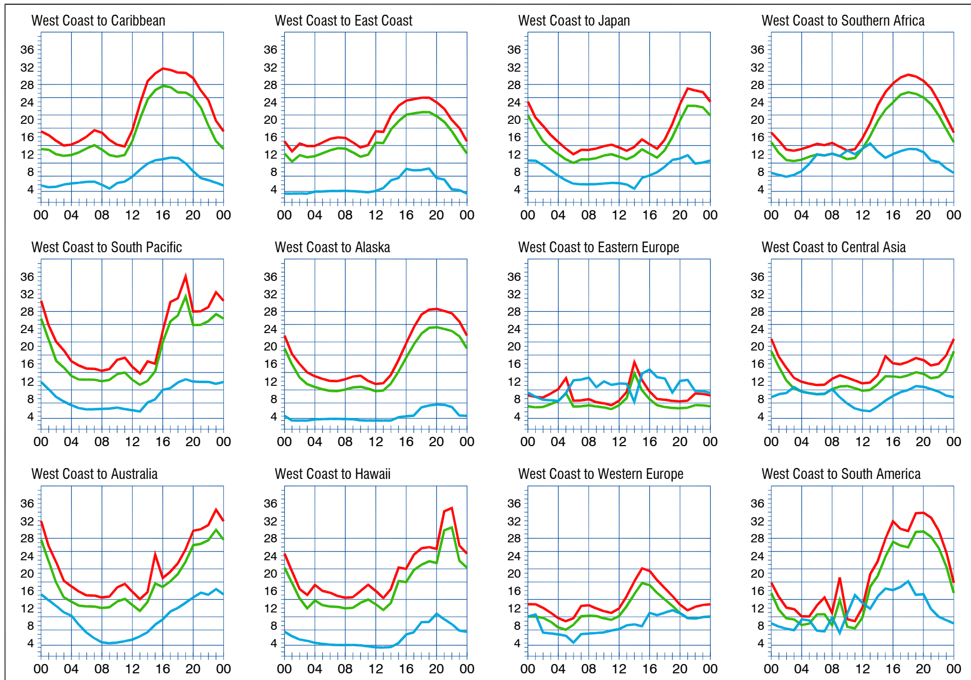
When are the bands open? These charts, generated using CAPman, show probabilities for average HF propagation in the month of November for the paths indicated. The horizontal axes show Coordinated Universal Time (UTC), and the vertical axes frequency in MHz. On 10% of the days of this period, the highest frequencies propagated will be at least as high as the upper red curves (HPF, highest possible frequency) and on 50% of the days they will be at least as high as the green curves (MUF, classical maximum usable frequency). The blue curves show the lowest usable frequency (LUF) for a 1500-W CW transmitter. For SSB or a lower transmitter power, the LUF will be somewhat higher than the blue curves indicate. See Oct 1994 QST , pp 27-30, and Feb 1995 QST , pp 34-36, for more details. The predictions assume an observed 2800-MHz solar flux value of 71. This is a Very Low level of solar activity. See the detailed propagation tables on The ARRL Antenna Book CD-ROM .
