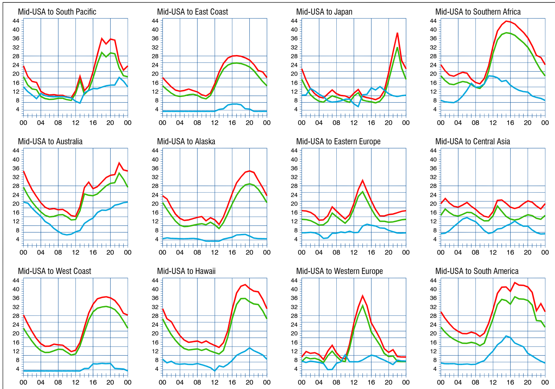
When are the bands open? These charts, generated using CAPman, show probabilities for average propagation in the Month of December. On 10% of the days of this period, the highest frequencies propagated will be at least as high as the upper red curves (HPF, highest possible frequency) and on 50% of the days they will be at least as high as the green curves (MUF, classical maximum usable frequency). The blue curves show the lowest usable frequency (LUF) for a 1500-W CW transmitter. For SSB or a lower power transmitter, the LUF will be somewhat higher than the blue curves indicate. The horizontal axes show Coordinated Universal Time (UTC) and the vertical axes frequency in MHz. These predictions assume an observed 2800-MHz solar flux value of 146
