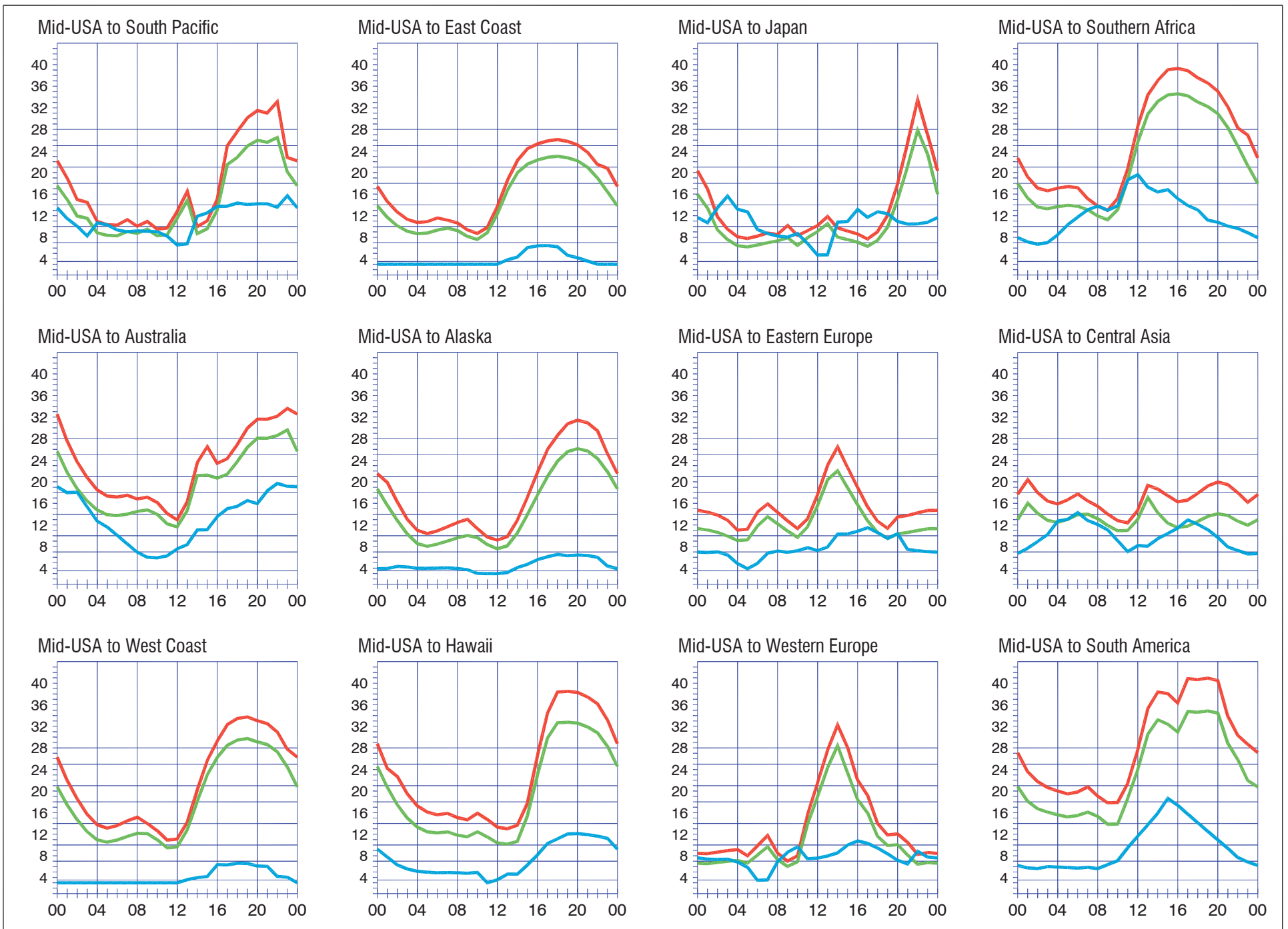
When are the bands open? These charts, generated using CAPman, show probabilities for average HF propagation in the month of January for the paths indicated. The horizontal axes show Coordinated Universal Time (UTC), and the vertical axes frequency in MHz. On 10 % of the days of this period, the highest frequencies propagated will be at least as high as the upper red curves (HPF, highest possible frequency) and on 50% of the days they will be at least as high as the green curves (MUF, classical maximum usable frequency). The blue curves show the lowest usable frequency (LUF) for a 1500-W CW transmitter. For SSB or a lower transmitter power, the LUF will be somewhat higher than the blue curves indicate. See Oct 1994 QST, pp 27-30, and Feb 1995 QST, pp 34-36, for more details. The predictions assume an observed 2800-MHz solar flux value of 124. This is a High level of solar activity. See the detailed propagation tables on The ARRL Antenna Book CD-ROM.
