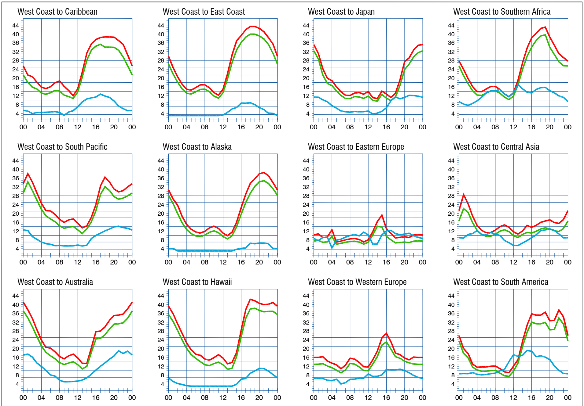
When are the bands open? These charts, generated using CAPman, show probabilities for average propagation in the Month of January. On 10% of the days of this period, the highest frequencies propagated will be at least as high as the upper red curves (HPF, highest possible frequency) and on 50% of the days they will be at least as high as the green curves (MUF, classical maximum usable frequency). The blue curves show the lowest usable frequency (LUF) for a 1500-W CW transmitter. For SSB or a lower power transmitter, the LUF will be somewhat higher than the blue curves indicate. The horizontal axes show Coordinated Universal Time (UTC) and the vertical axes frequency in MHz. These predictions assume an observed 2800-MHz solar flux value of 146.
