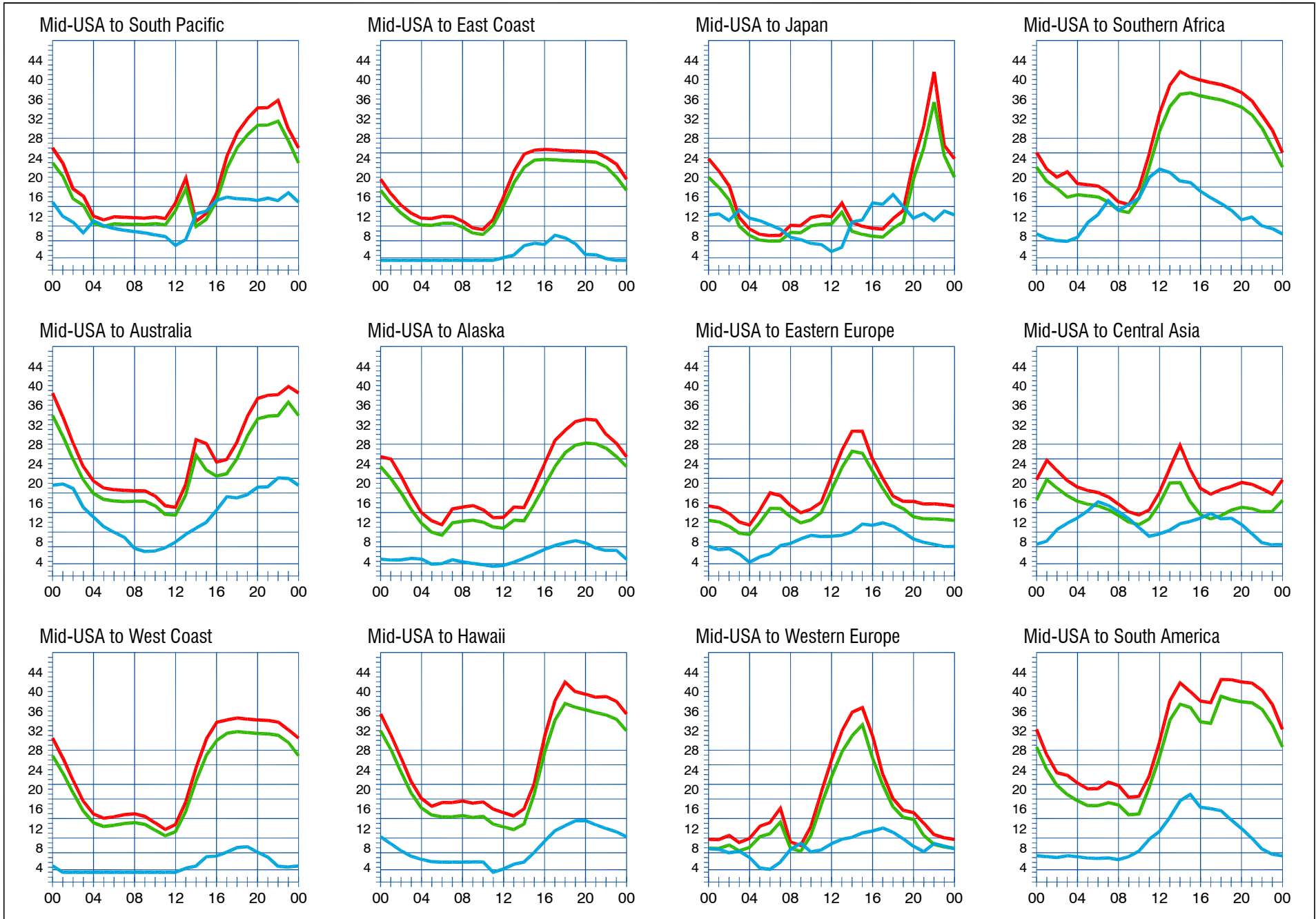
When are the bands open? These charts, generated using CAPman, show probabilities for average propagation in the Month of February. On 10% of the days of this period, the highest frequencies propagated will be at least as high as the upper red curves (HPF, highest possible frequency) and on 50% of the days they will be at least as high as the green curves (MUF, classical maximum usable frequency). The blue curves show the lowest usable frequency (LUF) for a 1500-W CW transmitter. For SSB or a lower power transmitter, the LUF will be somewhat higher than the blue curves indicate. The horizontal axes show Coordinated Universal Time (UTC) and the vertical axes frequency in MHz. These predictions assume an observed 2800-MHz solar flux value of 146.
