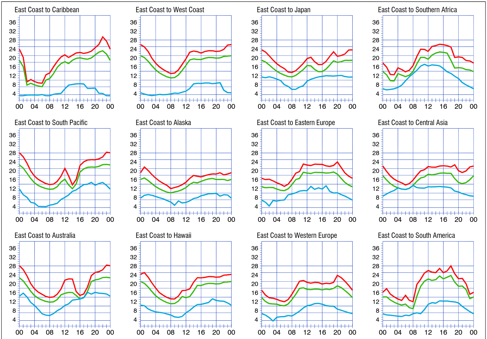
When are the bands open? These charts, generated using CAPman, show probabilities for average HF propagation in the month of May for the paths indicated. The horizontal axes show Coordinated Universal Time (UTC), and the vertical axes frequency in MHz. On 10% of the days of this period, the highest frequencies propagated will be at least as high as the upper red curves (HPF, highest possible frequency) and on 50% of the days they will be at least as high as the green curves (MUF, classical maximum usable frequency). The blue curves show the lowest usable frequency (LUF) for a 1500-W CW transmitter. For SSB or a lower transmitter power, the LUF will be somewhat higher than the blue curves indicate. See Oct 1994 QST , pp 27-30, and Feb 1995 QST , pp 34-36, for more details. The predictions assume an observed 2800-MHz solar flux value of 74. This is a Very Low level of solar activity. See the detailed propagation tables on The ARRL Antenna Book CD-ROM .
