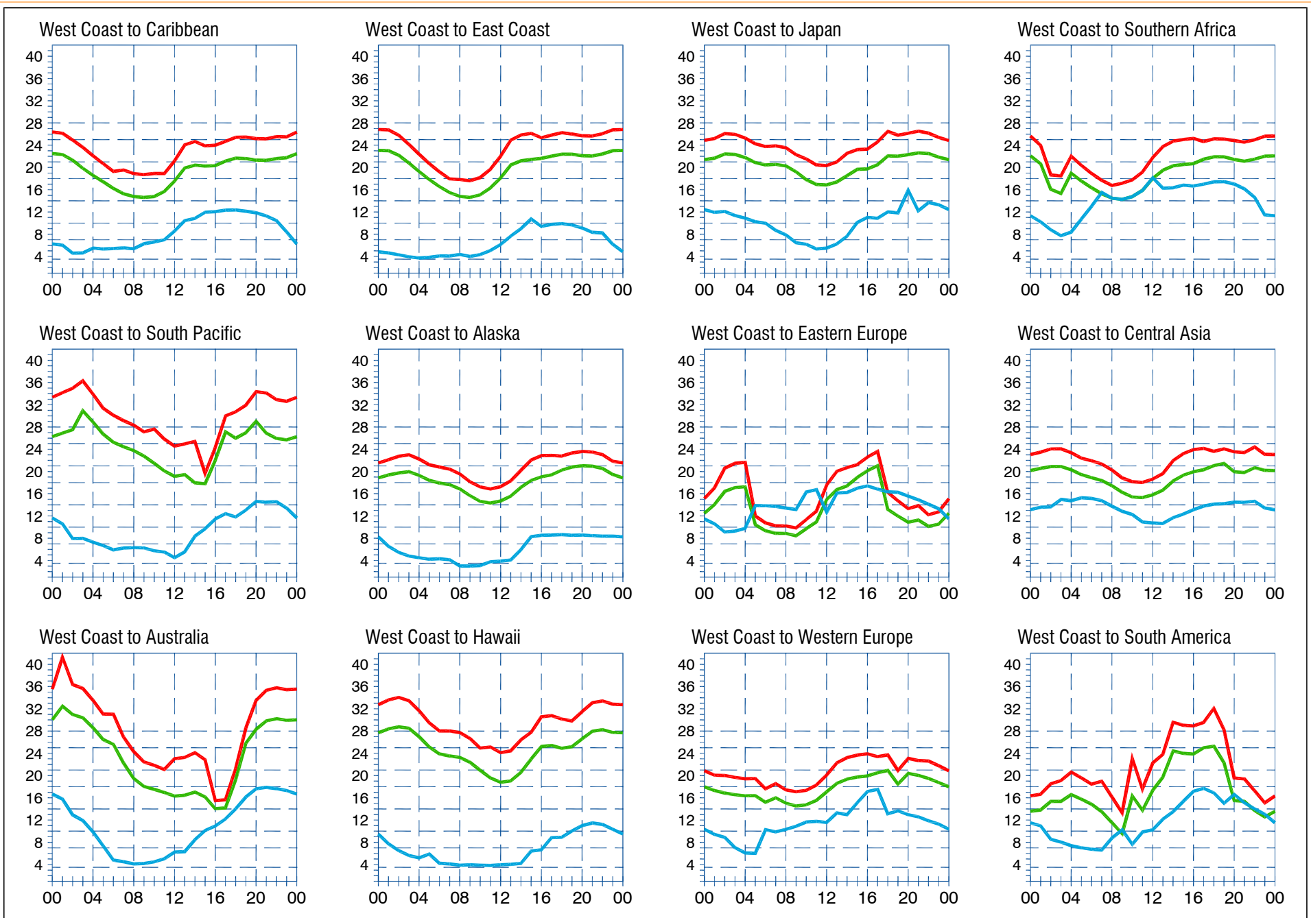
When are the bands open? These charts, generated using CAPman, show probabilities for average propagation in the Month of June. On 10% of the days of this period, the highest frequencies propagated will be at least as high as the upper red curves (HPF, highest possible frequency) and on 50% of the days they will be at least as high as the green curves (MUF, classical maximum usable frequency). The blue curves show the lowest usable frequency (LUF) for a 1500-W CW transmitter. For SSB or a lower power transmitter, the LUF will be somewhat higher than the blue curves indicate. The horizontal axes show Coordinated Universal Time (UTC) and the vertical axes frequency in MHz. These predictions assume an observed 2800-MHz solar flux value of 130.
