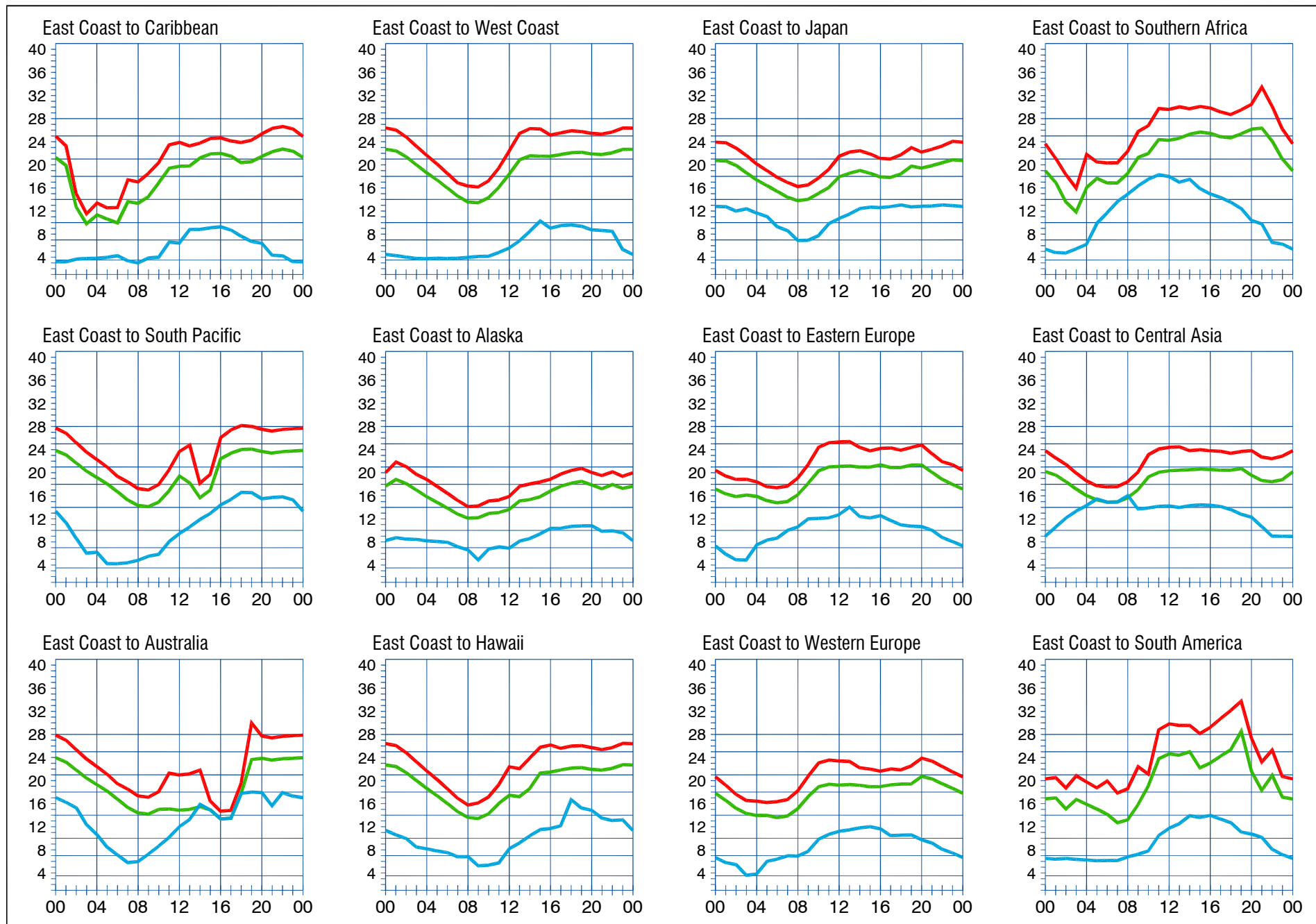
When are the bands open? These charts, generated using CAPman, show probabilities for average propagation in the Month of July. On 10% of the days of this period, the highest frequencies propagated will be at least as high as the upper red curves (HPF, highest possible frequency) and on 50% of the days they will be at least as high as the green curves (MUF, classical maximum usable frequency). The blue curves show the lowest usable frequency (LUF) for a 1500-W CW transmitter. For SSB or a lower power transmitter, the LUF will be somewhat higher than the blue curves indicate. The horizontal axes show Coordinated Universal Time (UTC) and the vertical axes frequency in MHz. These predictions assume an observed 2800-MHz solar flux value of 123.
