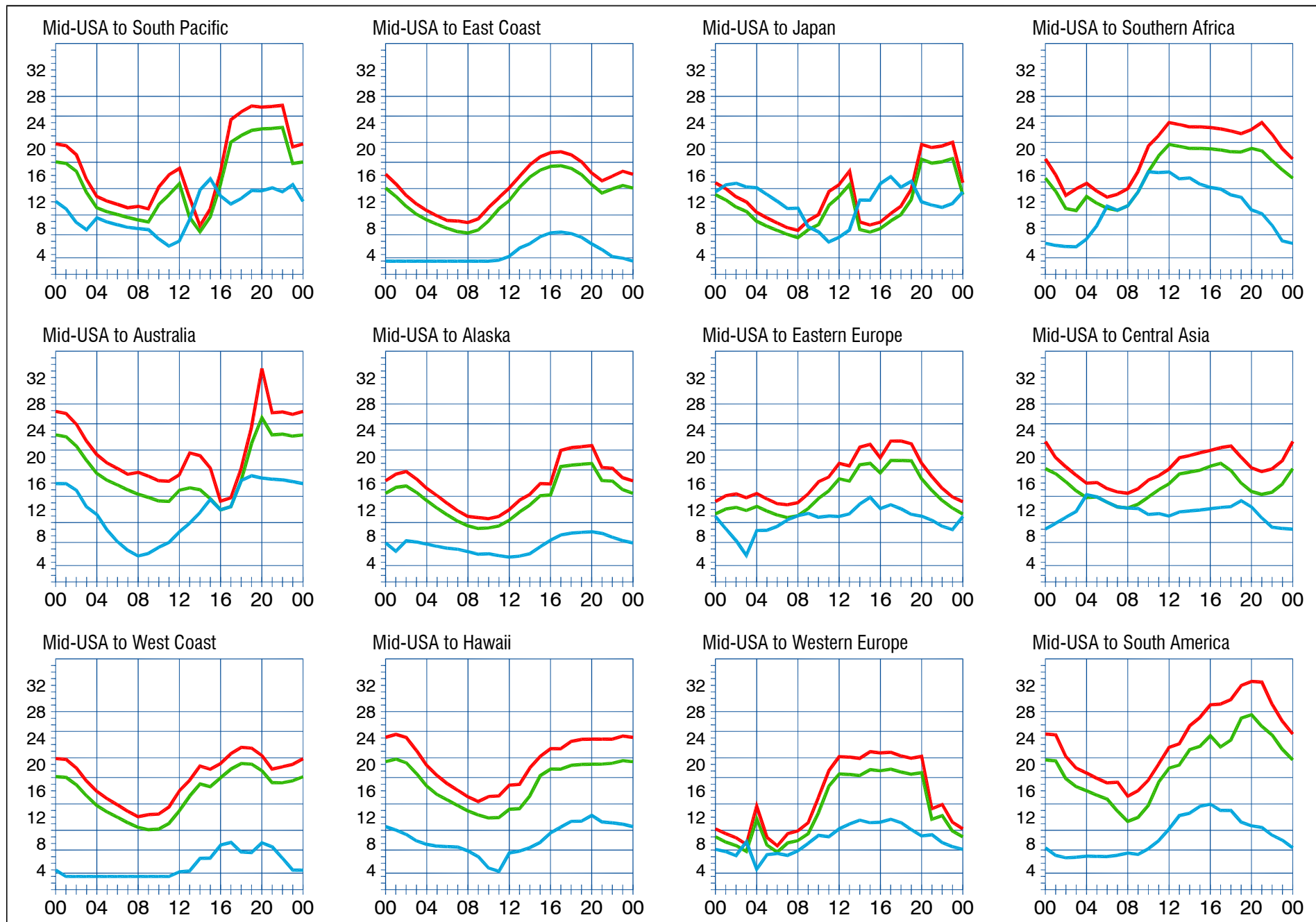
When are the bands open? These charts, generated using CAPman, show probabilities for average propagation in the Month of August. On 10% of the days of this period, the highest frequencies propagated will be at least as high as the upper red curves (HPF, highest possible frequency) and on 50% of the days they will be at least as high as the green curves (MUF, classical maximum usable frequency). The blue curves show the lowest usable frequency (LUF) for a 1500-W CW transmitter. For SSB or a lower power transmitter, the LUF will be somewhat higher than the blue curves indicate. The horizontal axes show Coordinated Universal Time (UTC) and the vertical axes frequency in MHz. These predictions assume an observed 2800-MHz solar flux value of 92.
