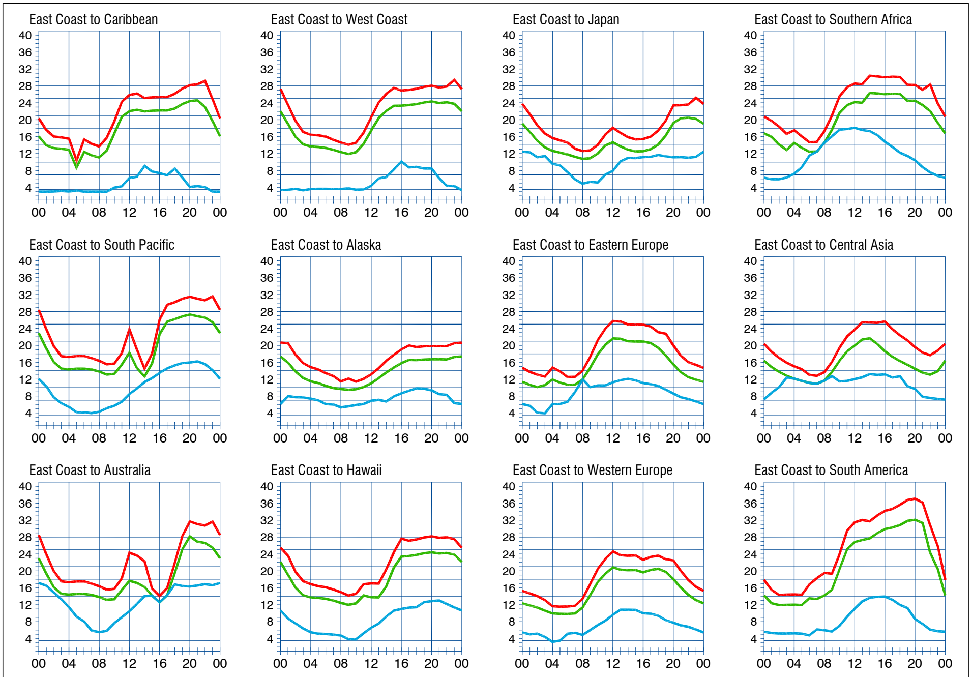
When are the bands open? These charts, generated using CAPman, show probabilities for average propagation in the Month of September. On 10% of the days of this period, the highest frequencies propagated will be at least as high as the upper red curves (HPF, highest possible frequency) and on 50% of the days they will be at least as high as the green curves (MUF, classical maximum usable frequency). The blue curves show the lowest usable frequency (LUF) for a 1500-W CW transmitter. For SSB or a lower power transmitter, the LUF will be somewhat higher than the blue curves indicate. The horizontal axes show Coordinated Universal Time (UTC) and the vertical axes frequency in MHz. These predictions assume an observed 2800-MHz solar flux value of 95.
