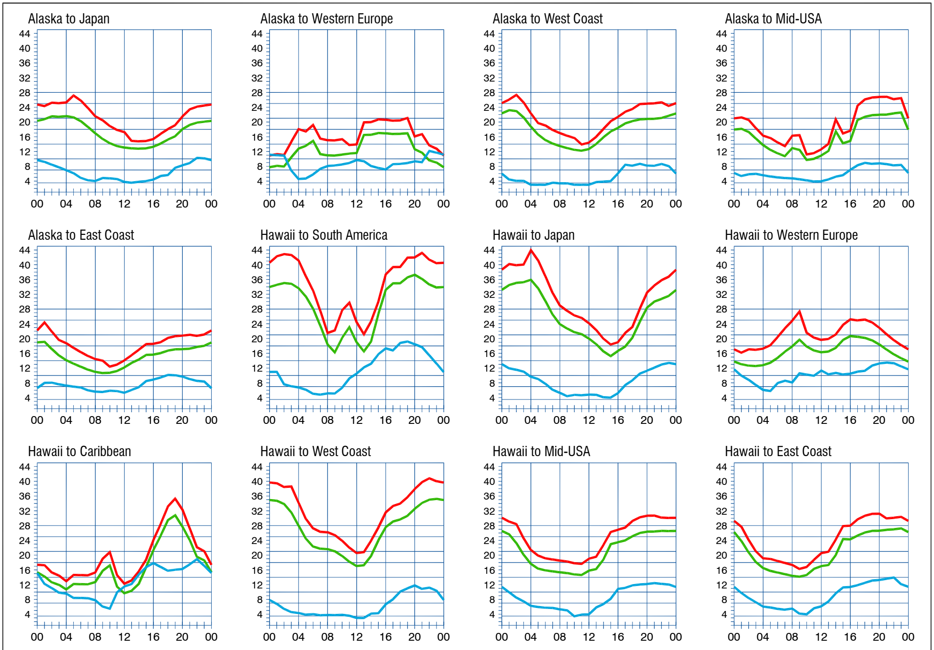
When are the bands open? These charts, generated using CAPman, show probabilities for average propagation in the Month of April. On 10% of the days of this period, the highest frequencies propagated will be at least as high as the upper red curves (HPF, highest possible frequency) and on 50% of the days they will be at least as high as the green curves (MUF, classical maximum usable frequency). The blue curves show the lowest usable frequency (LUF) for a 1500-W CW transmitter. For SSB or a lower power transmitter, the LUF will be somewhat higher than the blue curves indicate. The horizontal axes show Coordinated Universal Time (UTC) and the vertical axes frequency in MHz. These predictions assume an observed 2800-MHz solar flux value of 115.
