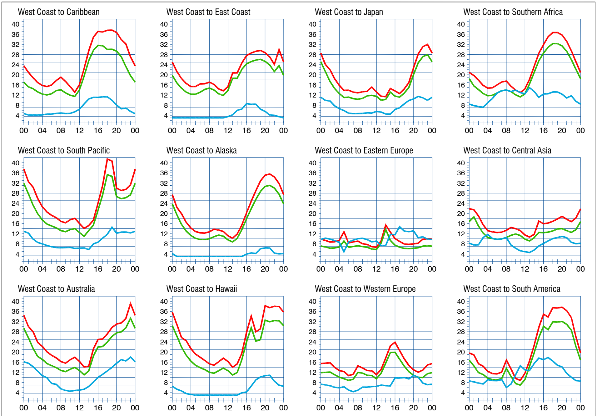
When are the bands open? These charts, generated using CAPman, show probabilities for average HF propagation in the month of December 2009 for the paths indicated. The horizontal axes show Coordinated Universal Time (UTC), and the vertical axes frequency in MHz. On 10% of the days of this period, the highest frequencies propagated will be at least as high as the upper red curves (HPF, highest possible frequency) and on 50% of the days they will be at least as high as the green curves (MUF, classical maximum usable frequency). The blue curves show the lowest usable frequency (LUF) for a 1500-W CW transmitter. For SSB or a lower transmitter power, the LUF will be somewhat higher than the blue curves indicate. See Oct 1994 QST , pp 27-30, and Feb 1995 QST , pp 34-36, for more details. The predictions assume an observed 2800-MHz solar flux value of 104. This is a Medium level of solar activity. See the detailed propagation tables on The ARRL Antenna Book CD-ROM .
