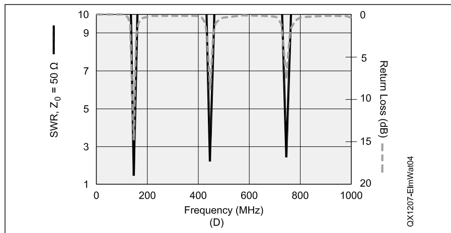
Figure 4D — This is the corrected version of Figure 4D from “A New Antenna Model,” Jul/Aug 2012 QEX, p 10. Note that the SWR scale along the left edge of the graph has been corrected to show an SWR of 1 at the bottom of the graph.
