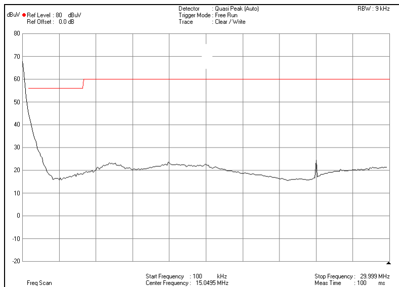
Recessed Grounded Metal Fixture Neutral
