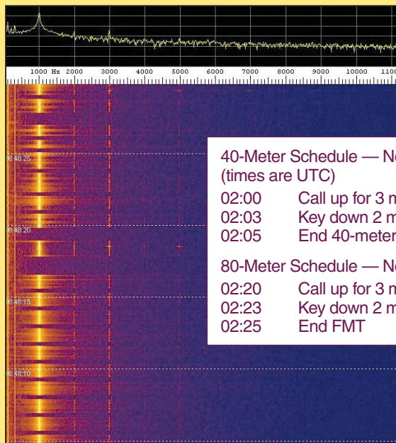
Measuring audio frequencies with Spectrum Lab .
