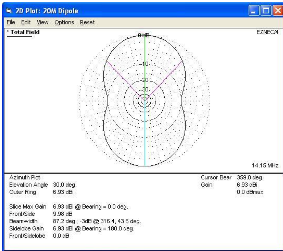
Figure 1: Azimuth pattern of a half wave dipole at a height of half a wave length has a -3 dB beamwidth of 87^\circ on each side -- a close match to the coverage needed by W1ZR to reach US and Canadian stations.
