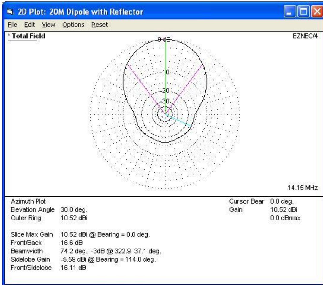
Figure 3 -- If I have no need for coverage to the rear, I can optimize the reflector length to achieve more gain by focusing almost all my signal to the front.
