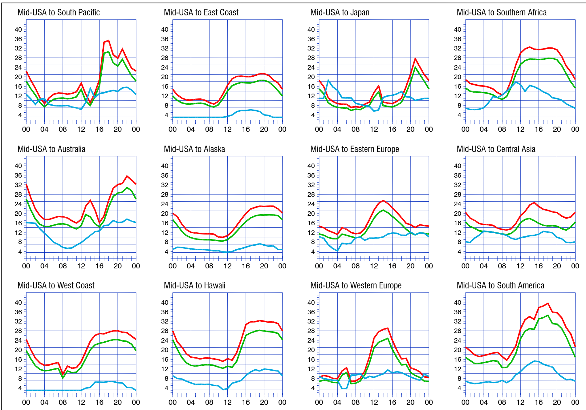
When are the bands open? These charts, generated using CAPman, show probabilities for average HF propagation in the month of October 2004 for the paths indicated. The horizontal axes show Coordinated Universal Time (UTC), and the vertical axes frequency in MHz. On 10 % of the days of this period, the highest frequencies propagated will be at least as high as the upper red curves (HPF, highest possible frequency) and on 50 % of the days they will be at least as high as the green curves (MUF, classical maximum usable frequency). The blue curves show the lowest usable frequency (LUF) for a 1500-W CW transmitter. For SSB or a lower transmitter power, the LUF will be somewhat higher than the blue curves indicate. See Oct 1994 QST, pp 27-30, and Feb 1995 QST, pp 34-36, for more details. The predictions assume an observed 2800-MHz solar flux value of 90. This is a Low level of solar activity. See the detailed propagation tables on The ARRL Antenna Book CD-ROM .
