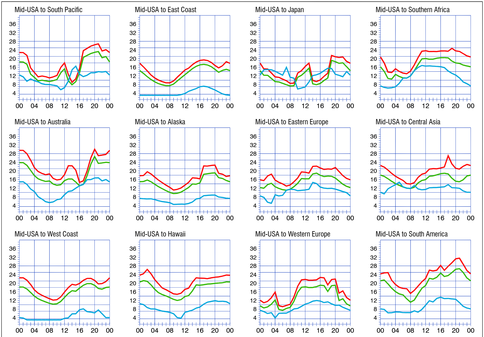
When are the bands open? These charts, generated using CAPman, show probabilities for average HF propagation in the month of May 2005 for the paths indicated. The horizontal axes show Coordinated Universal Time (UTC), and the vertical axes frequency in MHz. On 10% of the days of this period, the highest frequencies propagated will be at least as high as the upper red curves (HPF, highest possible frequency) and on 50% of the days they will be at least as high as the green curves (MUF, classical maximum usable frequency). The blue curves show the lowest usable frequency (LUF) for a 1500-W CW transmitter. For SSB or a lower transmitter power, the LUF will be somewhat higher than the blue curves indicate. See Oct 1994 QST , pp 27-30, and Feb 1995 QST , pp 34-36, for more details. The predictions assume an observed 2800-MHz solar flux value of 82. This is a Low level of solar activity. See the detailed propagation tables on The ARRL Antenna Book CD-ROM .
