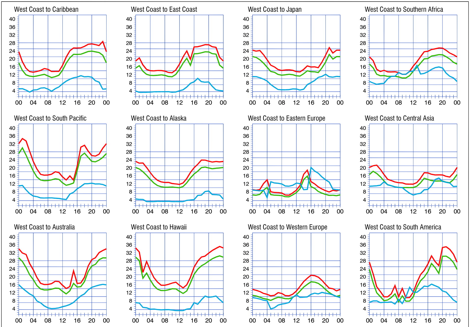
When are the bands open? These charts, generated using CAPman, show probabilities for average HF propagation in the month of March 2007 for the paths indicated. The horizontal axes show Coordinated Universal Time (UTC), and the vertical axes frequency in MHz. On 10% of the days of this period, the highest frequencies propagated will be at least as high as the upper red curves (HPF, highest possible frequency) and on 50% of the days they will be at least as high as the green curves (MUF, classical maximum usable frequency). The blue curves show the lowest usable frequency (LUF) for a 1500-W CW transmitter. For SSB or a lower transmitter power, the LUF will be somewhat higher than the blue curves indicate. See Oct 1994 QST , pp 27-30, and Feb 1995 QST , pp 34-36, for more details. The predictions assume an observed 2800-MHz solar flux value of 73. This is a Very Low level of solar activity. See the detailed propagation tables on The ARRL Antenna Book CD-ROM .
