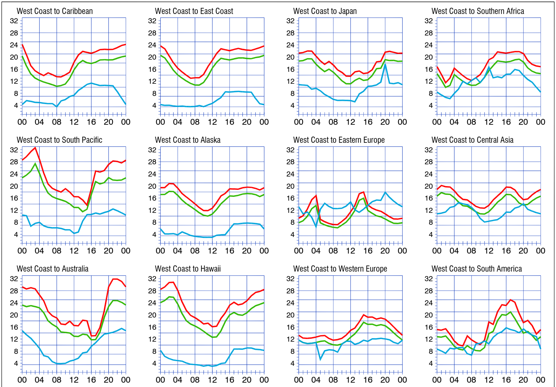
When are the bands open? These charts, generated using CAPman, show probabilities for average HF propagation in the month of August 2007 for the paths indicated. The horizontal axes show Coordinated Universal Time (UTC), and the vertical axes frequency in MHz. On 10% of the days of this period, the highest frequencies propagated will be at least as high as the upper red curves (HPF, highest possible frequency) and on 50% of the days they will be at least as high as the green curves (MUF, classical maximum usable frequency). The blue curves show the lowest usable frequency (LUF) for a 1500-W CW transmitter. For SSB or a lower transmitter power, the LUF will be somewhat higher than the blue curves indicate. See Oct 1994 QST , pp 27-30, and Feb 1995 QST , pp 34-36, for more details. The predictions assume an observed 2800-MHz solar flux value of 76. This is a Very Low level of solar activity. See the detailed propagation tables on The ARRL Antenna Book CD-ROM .
