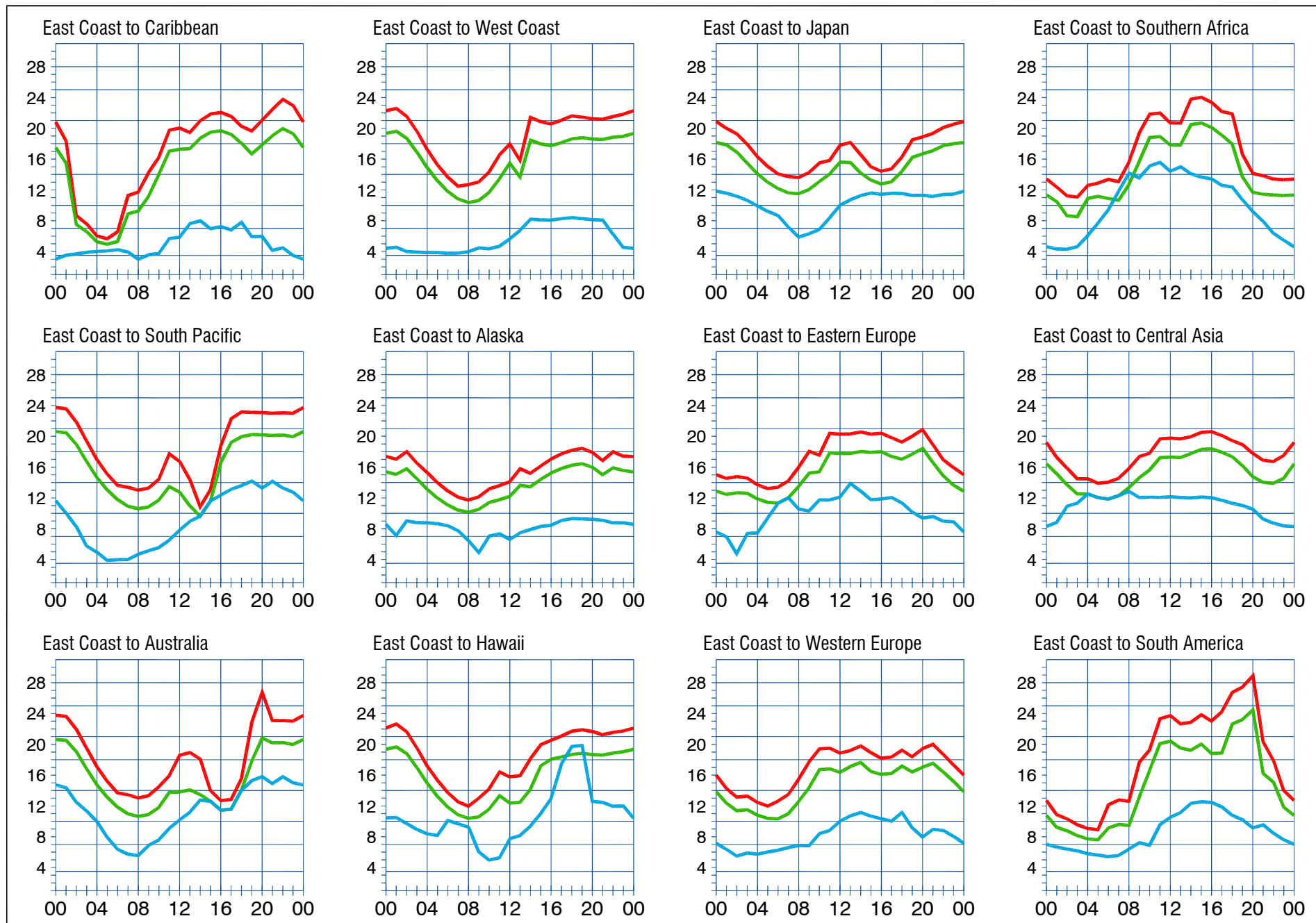
When are the bands open? These charts, generated using CAPman, show probabilities for average HF propagation in the month of July 2008 for the paths indicated. The horizontal axes show Coordinated Universal Time (UTC), and the vertical axes frequency in MHz. On 10% of the days of this period, the highest frequencies propagated will be at least as high as the upper red curves (HPF, highest possible frequency) and on 50% of the days they will be at least as high as the green curves (MUF, classical maximum usable frequency). The blue curves show the lowest usable frequency (LUF) for a 1500-W CW transmitter. For SSB or a lower transmitter power, the LUF will be somewhat higher than the blue curves indicate. See Oct 1994 QST , pp 27-30, and Feb 1995 QST , pp 34-36, for more details. The predictions assume an observed 2800-MHz solar flux value of 67. This is a Very Low level of solar activity. See the detailed propagation tables on The ARRL Antenna Book CD-ROM .
