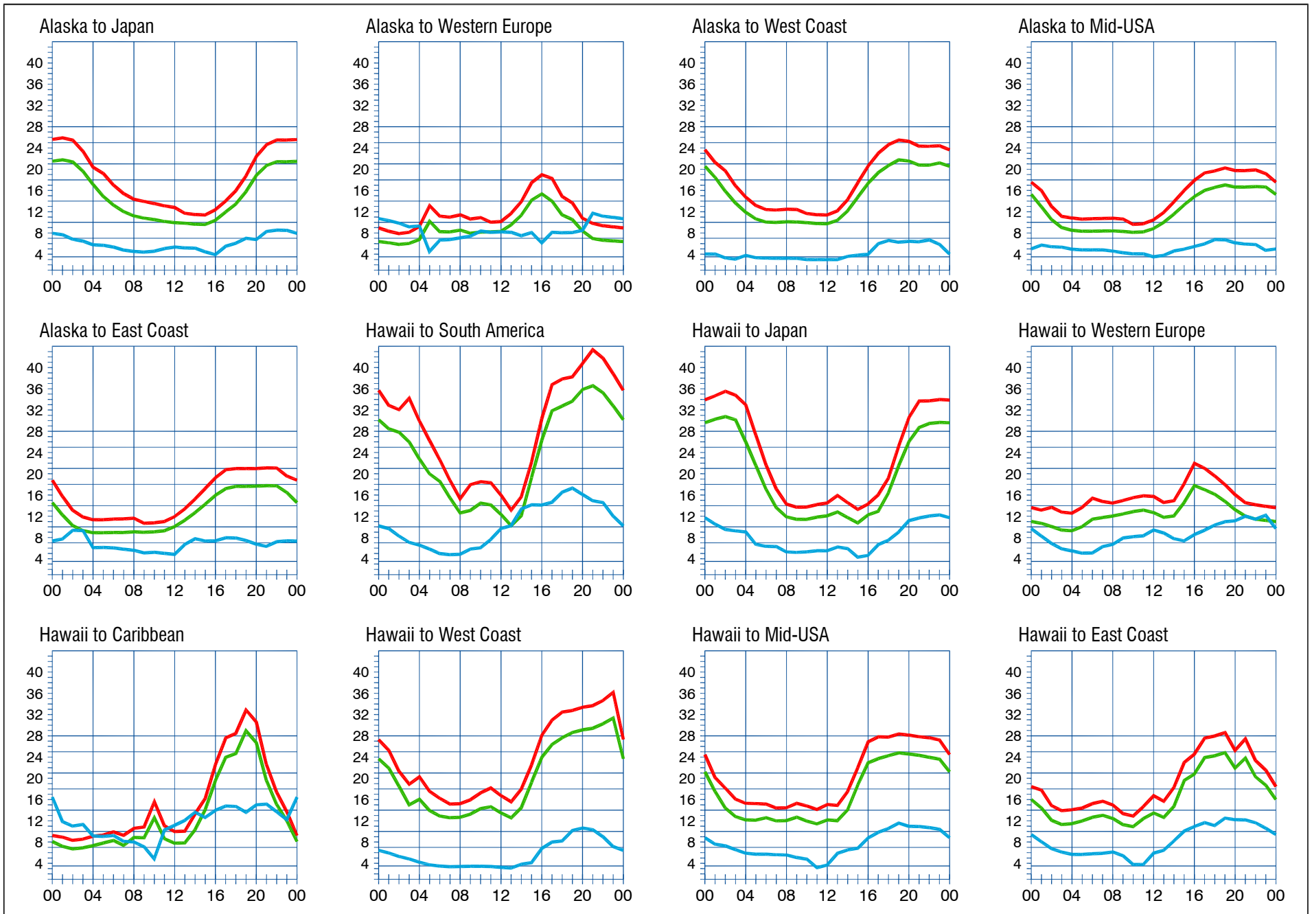
When are the bands open? These charts, generated using CAPman, show probabilities for average HF propagation in the month of October 2008 for the paths indicated. The horizontal axes show Coordinated Universal Time (UTC), and the vertical axes frequency in MHz. On 10% of the days of this period, the highest frequencies propagated will be at least as high as the upper red curves (HPF, highest possible frequency) and on 50% of the days they will be at least as high as the green curves (MUF, classical maximum usable frequency). The blue curves show the lowest usable frequency (LUF) for a 1500-W CW transmitter. For SSB or a lower transmitter power, the LUF will be somewhat higher than the blue curves indicate. See Oct 1994 QST , pp 27-30, and Feb 1995 QST , pp 34-36, for more details. The predictions assume an observed 2800-MHz solar flux value of 70. This is a Very Low level of solar activity. See the detailed propagation tables on The ARRL Antenna Book CD-ROM .
