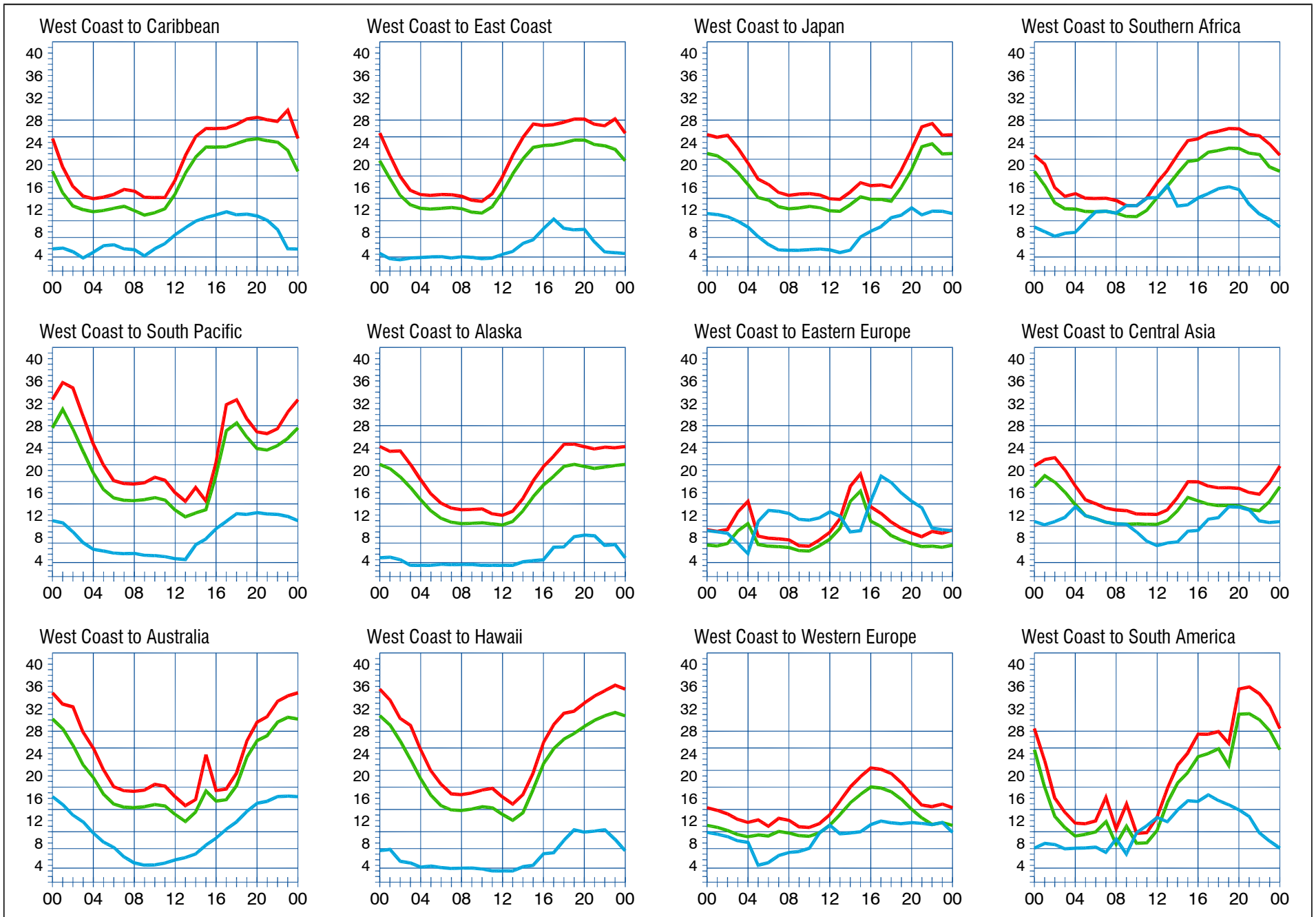
When are the bands open? These charts, generated using CAPman, show probabilities for average HF propagation in the month of March 2009 for the paths indicated. The horizontal axes show Coordinated Universal Time (UTC), and the vertical axes frequency in MHz. On 10% of the days of this period, the highest frequencies propagated will be at least as high as the upper red curves (HPF, highest possible frequency) and on 50% of the days they will be at least as high as the green curves (MUF, classical maximum usable frequency). The blue curves show the lowest usable frequency (LUF) for a 1500-W CW transmitter. For SSB or a lower transmitter power, the LUF will be somewhat higher than the blue curves indicate. See Oct 1994 QST , pp 27-30, and Feb 1995 QST , pp 34-36, for more details. The predictions assume an observed 2800-MHz solar flux value of 79. This is a Low level of solar activity. See the detailed propagation tables on The ARRL Antenna Book CD-ROM .
