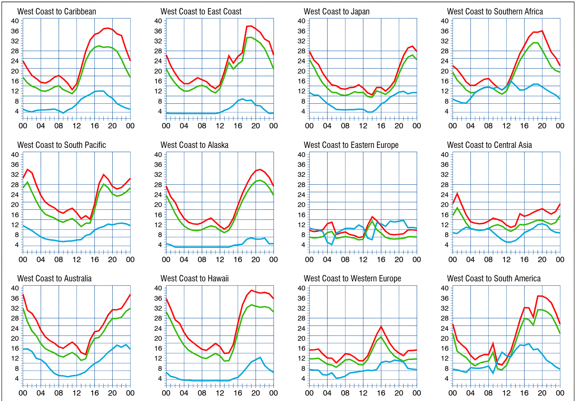
When are the bands open? These charts, generated using CAPman, show probabilities for average HF propagation in the month of January 2010 for the paths indicated. The horizontal axes show Coordinated Universal Time (UTC), and the vertical axes frequency in MHz. On 10% of the days of this period, the highest frequencies propagated will be at least as high as the upper red curves (HPF, highest possible frequency) and on 50% of the days they will be at least as high as the green curves (MUF, classical maximum usable frequency). The blue curves show the lowest usable frequency (LUF) for a 1500-W CW transmitter. For SSB or a lower transmitter power, the LUF will be somewhat higher than the blue curves indicate. See Oct 1994 QST , pp 27-30, and Feb 1995 QST , pp 34-36, for more details. The predictions assume an observed 2800-MHz solar flux value of 107. This is a Medium level of solar activity. See the detailed propagation tables on The ARRL Antenna Book CD-ROM .
