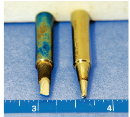
Figure 3 — The Mini Iron pencil tip (right) is preferred over a flat, wide soldering station tip (left). [Paul Cianciolo, W1VLF, photo]
