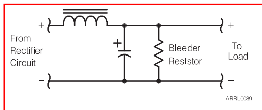
Figure G7-1 — This figure is used for questions G7A09 through G7A13.
