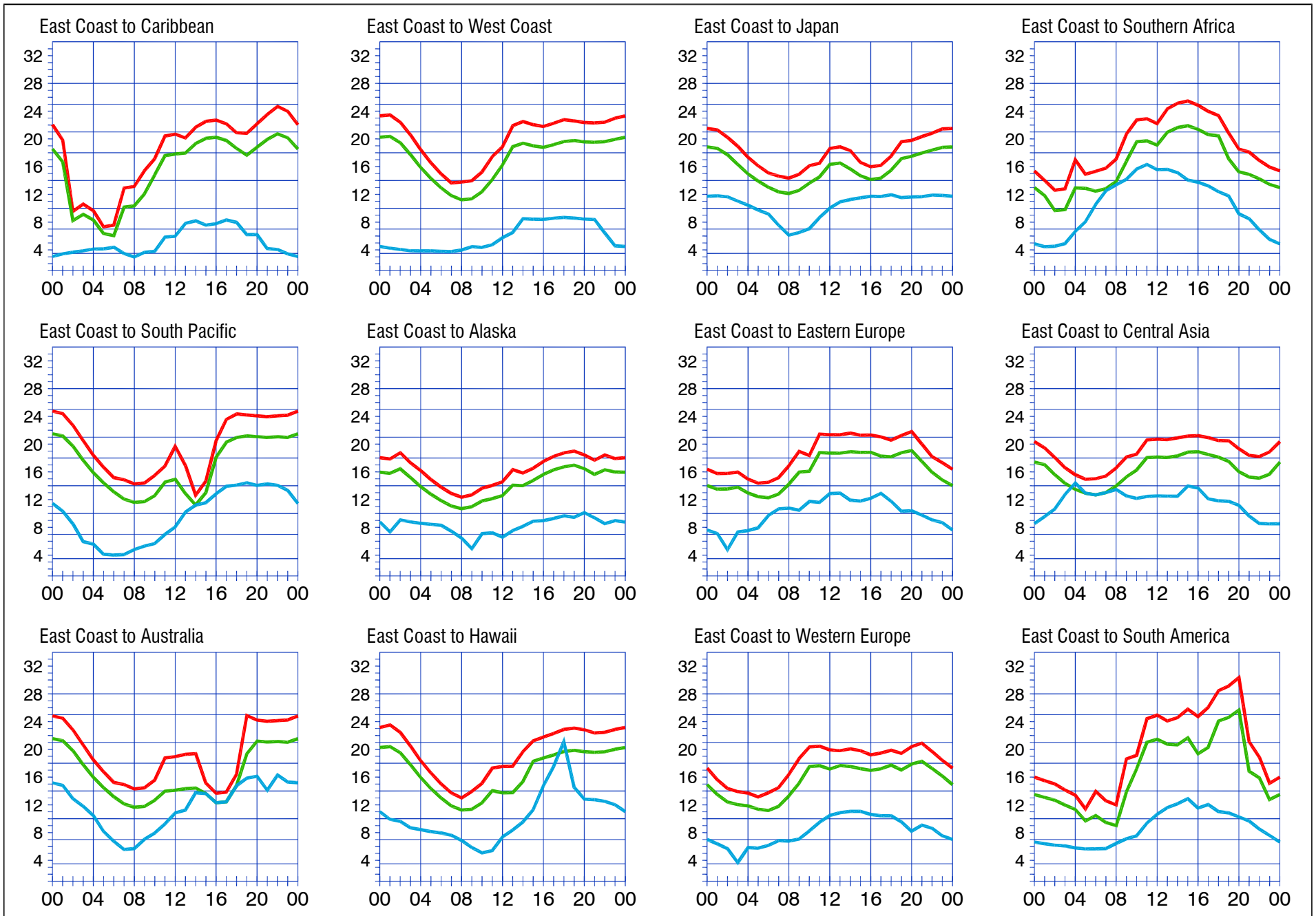
When are the bands open? These charts, generated using CAPman, show probabilities for average HF propagation in the month of July 2005 for the paths indicated. The horizontal axes show Coordinated Universal Time (UTC), and the vertical axes frequency in MHz. On 10% of the days of this period, the highest frequencies propagated will be at least as high as the upper red curves (HPF, highest possible frequency) and on 50% of the days they will be at least as high as the green curves (MUF, classical maximum usable frequency). The blue curves show the lowest usable frequency (LUF) for a 1500-W CW transmitter. For SSB or a lower transmitter power, the LUF will be somewhat higher than the blue curves indicate. See Oct 1994 QST , pp 27-30, and Feb 1995 QST , pp 34-36, for more details. The predictions assume an observed 2800-MHz solar flux value of 81. This is a Low level of solar activity. See the detailed propagation tables on The ARRL Antenna Book CD-ROM .
