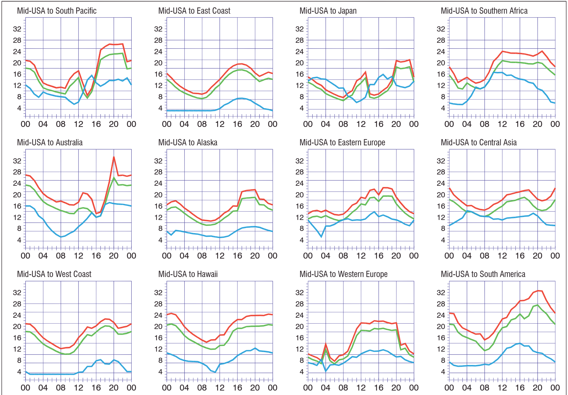
When are the bands open? These charts, generated using CAPman, show probabilities for average HF propagation in the month of August 2004 for the paths indicated. The horizontal axes show Coordinated Universal Time (UTC), and the vertical axes frequency in MHz. On 10 % of the days of this period, the highest frequencies propagated will be at least as high as the upper red curves (HPF, highest possible frequency) and on 50 % of the days they will be at least as high as the green curves (MUF, classical maximum usable frequency). The blue curves show the lowest usable frequency (LUF) for a 1500-W CW transmitter. For SSB or a lower transmitter power, the LUF will be somewhat higher than the blue curves indicate. See Oct 1994 QST , pp 27-30, and Feb 1995 QST , pp 34-36, for more details. The predictions assume an observed 2800-MHz solar flux value of 92. This is a Low level of solar activity. See the detailed propagation tables on The ARRL Antenna Book CD-ROM .
