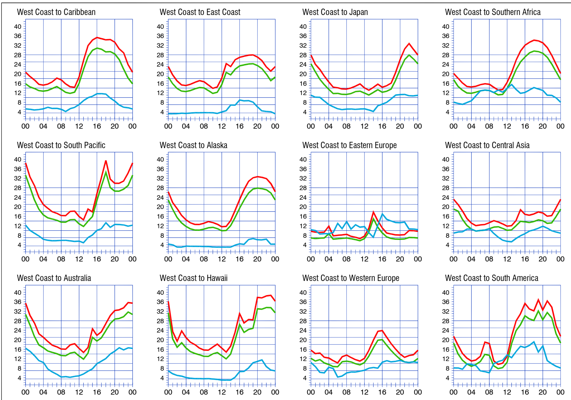
When are the bands open? These charts, generated using CAPman, show probabilities for average HF propagation in the month of November 2004 for the paths indicated. The horizontal axes show Coordinated Universal Time (UTC), and the vertical axes frequency in MHz. On 10 % of the days of this period, the highest frequencies propagated will be at least as high as the upper red curves (HPF, highest possible frequency) and on 50 % of the days they will be at least as high as the green curves (MUF, classical maximum usable frequency). The blue curves show the lowest usable frequency (LUF) for a 1500-W CW transmitter. For SSB or a lower transmitter power, the LUF will be somewhat higher than the blue curves indicate. See Oct 1994 QST , pp 27-30, and Feb 1995 QST , pp 34-36, for more details. The predictions assume an observed 2800-MHz solar flux value of 89. This is a Low level of solar activity. See the detailed propagation tables on The ARRL Antenna Book CD-ROM .
