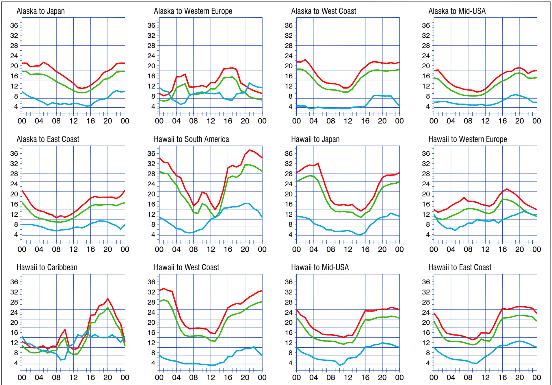
When are the bands open? These charts, generated using CAPman, show probabilities for average HF propagation in the month of September 2005 for the paths indicated. The horizontal axes show Coordinated Universal Time (UTC), and the vertical axes frequency in MHz. On 10% of the days of this period, the highest frequencies propagated will be at least as high as the upper red curves (HPF, highest possible frequency) and on 50% of the days they will be at least as high as the green curves (MUF, classical maximum usable frequency). The blue curves show the lowest usable frequency (LUF) for a 1500-W CW transmitter. For SSB or a lower transmitter power, the LUF will be somewhat higher than the blue curves indicate. See Oct 1994 QST , pp 27-30, and Feb 1995 QST , pp 34-36, for more details. The predictions assume an observed 2800-MHz solar flux value of 80. This is a Low level of solar activity. See the detailed propagation tables on The ARRL Antenna Book CD-ROM .
