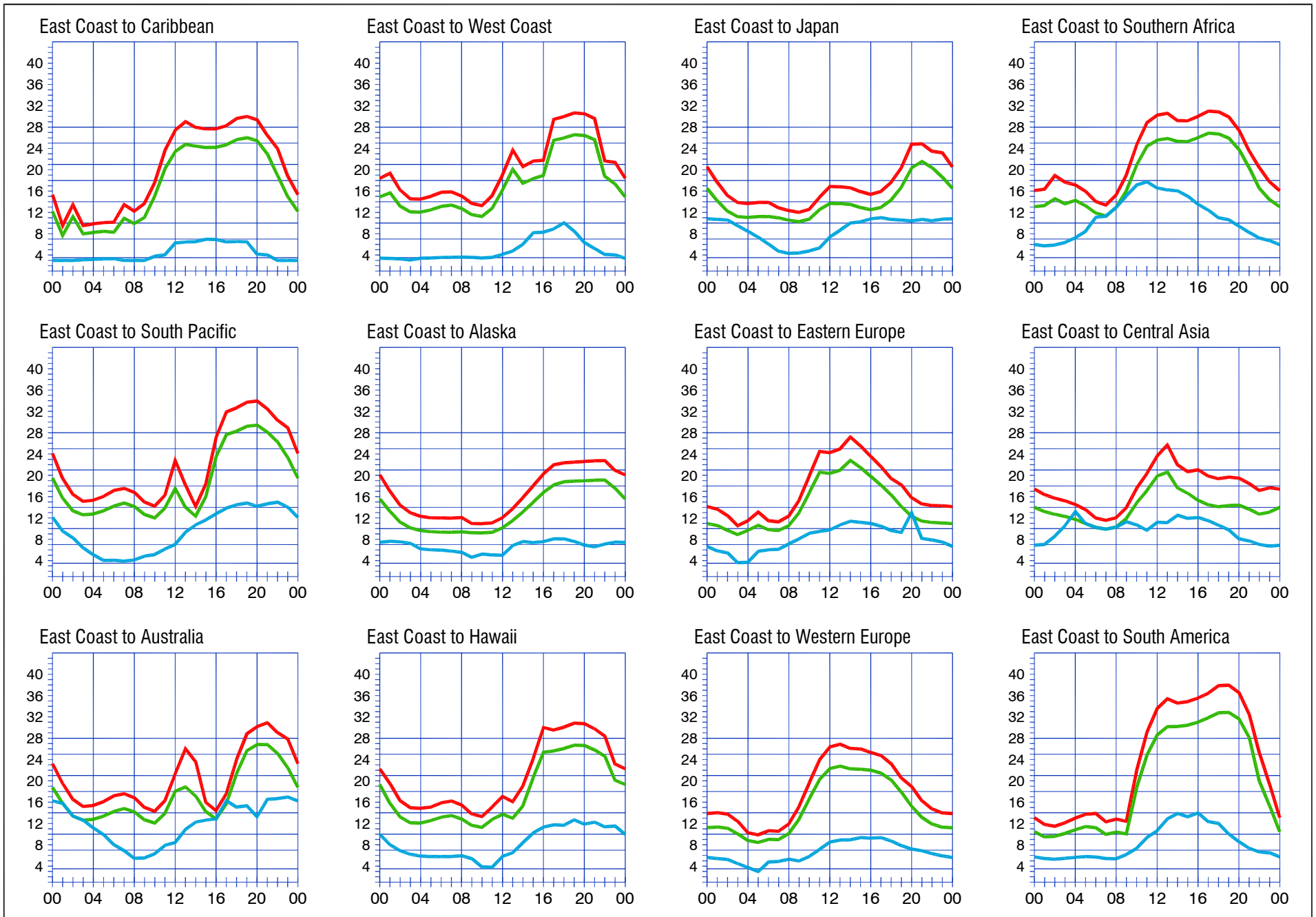
When are the bands open? These charts, generated using CAPman, show probabilities for average HF propagation in the month of October 2005 for the paths indicated. The horizontal axes show Coordinated Universal Time (UTC), and the vertical axes frequency in MHz. On 10% of the days of this period, the highest frequencies propagated will be at least as high as the upper red curves (HPF, highest possible frequency) and on 50% of the days they will be at least as high as the green curves (MUF, classical maximum usable frequency). The blue curves show the lowest usable frequency (LUF) for a 1500-W CW transmitter. For SSB or a lower transmitter power, the LUF will be somewhat higher than the blue curves indicate. See Oct 1994 QST , pp 27-30, and Feb 1995 QST , pp 34-36, for more details. The predictions assume an observed 2800-MHz solar flux value of 79. This is a Very Low level of solar activity. See the detailed propagation tables on The ARRL Antenna Book CD-ROM .
