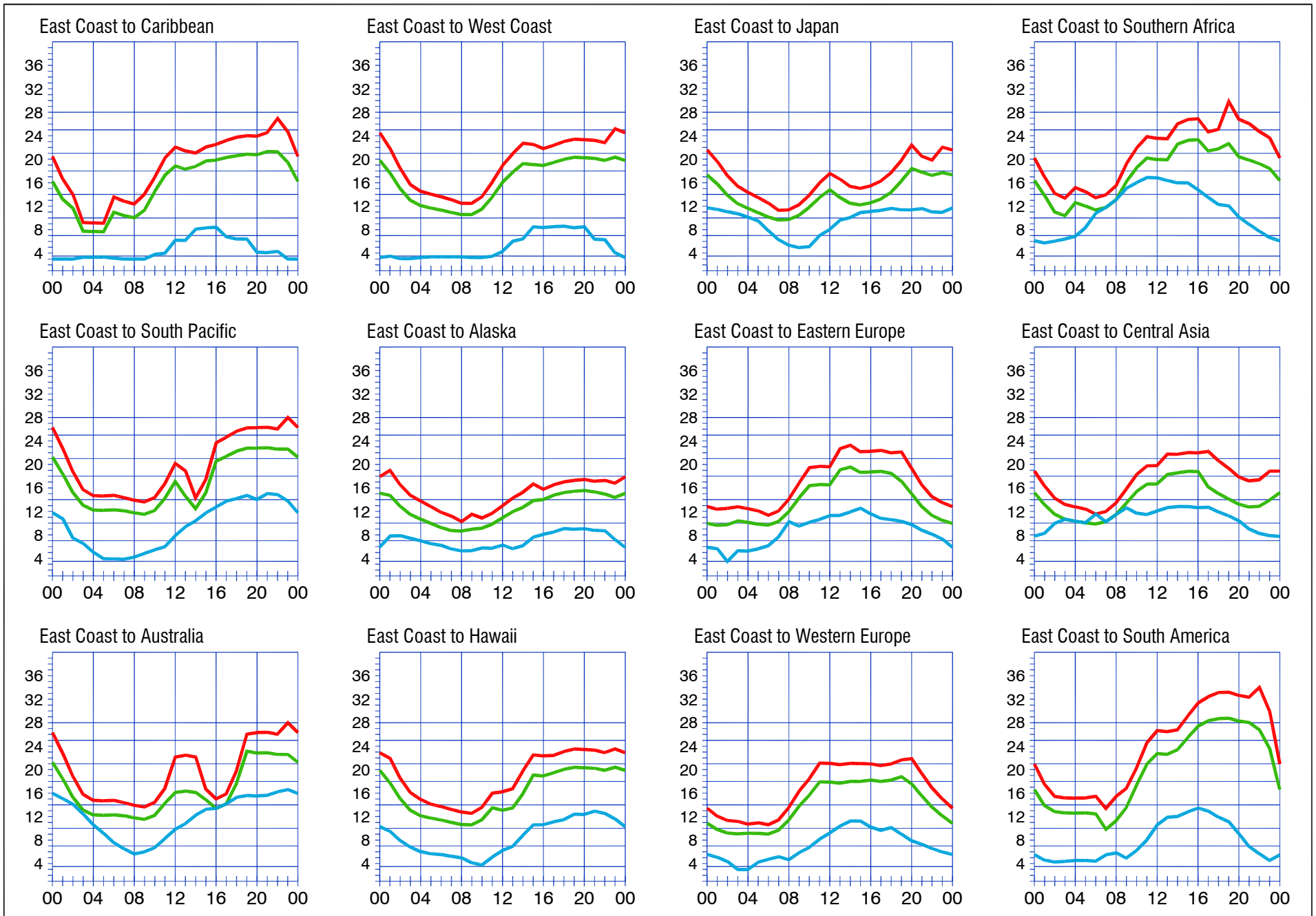
When are the bands open? These charts, generated using CAPman, show probabilities for average HF propagation in the month of April 2007 for the paths indicated. The horizontal axes show Coordinated Universal Time (UTC), and the vertical axes frequency in MHz. On 10% of the days of this period, the highest frequencies propagated will be at least as high as the upper red curves (HPF, highest possible frequency) and on 50% of the days they will be at least as high as the green curves (MUF, classical maximum usable frequency). The blue curves show the lowest usable frequency (LUF) for a 1500-W CW transmitter. For SSB or a lower transmitter power, the LUF will be somewhat higher than the blue curves indicate. See Oct 1994 QST , pp 27-30, and Feb 1995 QST , pp 34-36, for more details. The predictions assume an observed 2800-MHz solar flux value of 73. This is a Very Low level of solar activity. See the detailed propagation tables on The ARRL Antenna Book CD-ROM .
