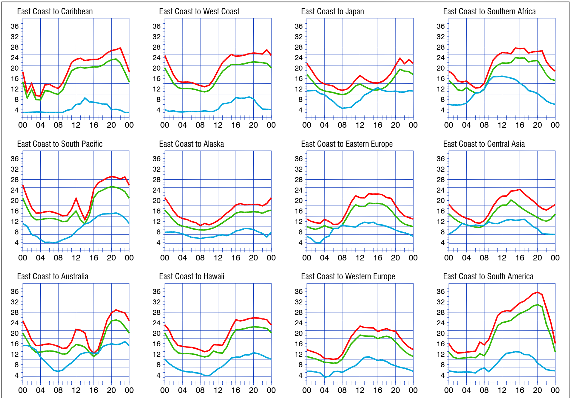
When are the bands open? These charts, generated using CAPman, show probabilities for average HF propagation in the month of September 2007 for the paths indicated. The horizontal axes show Coordinated Universal Time (UTC), and the vertical axes frequency in MHz. On 10% of the days of this period, the highest frequencies propagated will be at least as high as the upper red curves (HPF, highest possible frequency) and on 50% of the days they will be at least as high as the green curves (MUF, classical maximum usable frequency). The blue curves show the lowest usable frequency (LUF) for a 1500-W CW transmitter. For SSB or a lower transmitter power, the LUF will be somewhat higher than the blue curves indicate. See Oct 1994 QST , pp 27-30, and Feb 1995 QST , pp 34-36, for more details. The predictions assume an observed 2800-MHz solar flux value of 77. This is a Very Low level of solar activity. See the detailed propagation tables on The ARRL Antenna Book CD-ROM .
