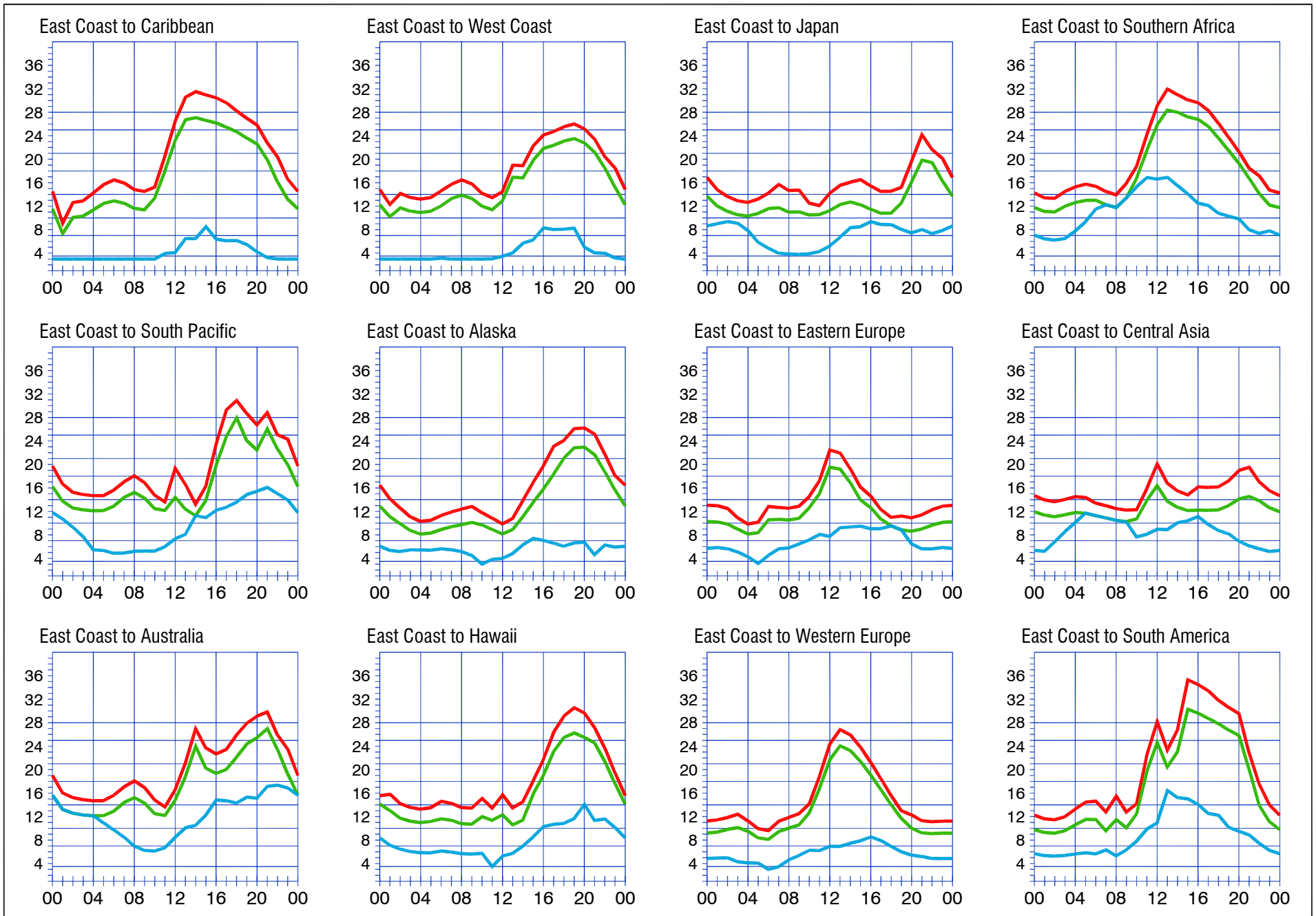
When are the bands open? These charts, generated using CAPman, show probabilities for average HF propagation in the month of December 2007 for the paths indicated. The horizontal axes show Coordinated Universal Time (UTC), and the vertical axes frequency in MHz. On 10% of the days of this period, the highest frequencies propagated will be at least as high as the upper red curves (HPF, highest possible frequency) and on 50% of the days they will be at least as high as the green curves (MUF, classical maximum usable frequency). The blue curves show the lowest usable frequency (LUF) for a 1500-W CW transmitter. For SSB or a lower transmitter power, the LUF will be somewhat higher than the blue curves indicate. See Oct 1994 QST , pp 27-30, and Feb 1995 QST , pp 34-36, for more details. The predictions assume an observed 2800-MHz solar flux value of 80. This is a Very Low level of solar activity. See the detailed propagation tables on The ARRL Antenna Book CD-ROM .
