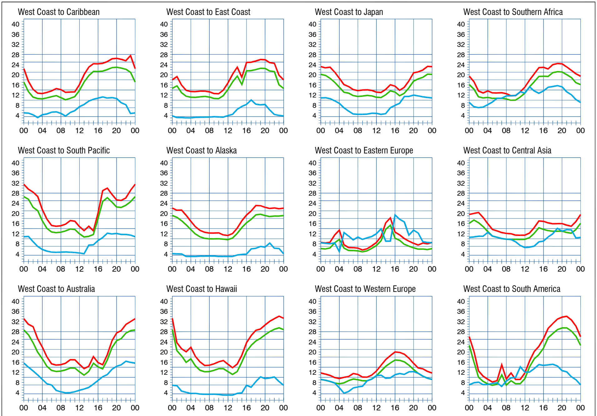
When are the bands open? These charts, generated using CAPman, show probabilities for average HF propagation in the month of March 2008 for the paths indicated. The horizontal axes show Coordinated Universal Time (UTC), and the vertical axes frequency in MHz. On 10% of the days of this period, the highest frequencies propagated will be at least as high as the upper red curves (HPF, highest possible frequency) and on 50% of the days they will be at least as high as the green curves (MUF, classical maximum usable frequency). The blue curves show the lowest usable frequency (LUF) for a 1500-W CW transmitter. For SSB or a lower transmitter power, the LUF will be somewhat higher than the blue curves indicate. See Oct 1994 QST , pp 27-30, and Feb 1995 QST , pp 34-36, for more details. The predictions assume an observed 2800-MHz solar flux value of 67. This is a Very Low level of solar activity. See the detailed propagation tables on The ARRL Antenna Book CD-ROM .
