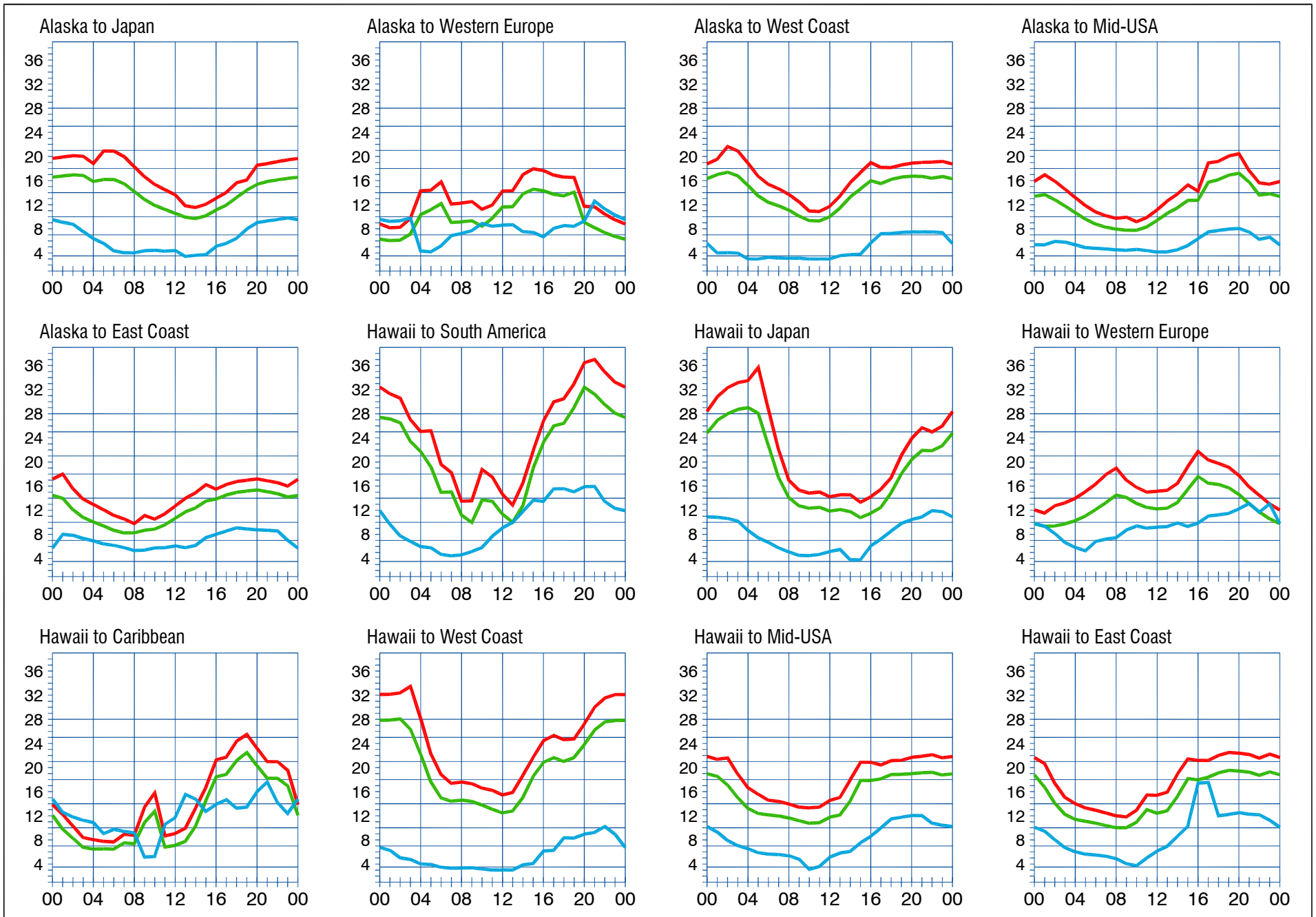
When are the bands open? These charts, generated using CAPman, show probabilities for average HF propagation in the month of April 2008 for the paths indicated. The horizontal axes show Coordinated Universal Time (UTC), and the vertical axes frequency in MHz. On 10% of the days of this period, the highest frequencies propagated will be at least as high as the upper red curves (HPF, highest possible frequency) and on 50% of the days they will be at least as high as the green curves (MUF, classical maximum usable frequency). The blue curves show the lowest usable frequency (LUF) for a 1500-W CW transmitter. For SSB or a lower transmitter power, the LUF will be somewhat higher than the blue curves indicate. See Oct 1994 QST , pp 27-30, and Feb 1995 QST , pp 34-36, for more details. The predictions assume an observed 2800-MHz solar flux value of 67. This is a Very Low level of solar activity. See the detailed propagation tables on The ARRL Antenna Book CD-ROM .
