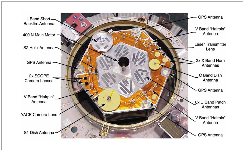
Fig 23.38—The various antennas that comprise AO-40's antenna farm.
